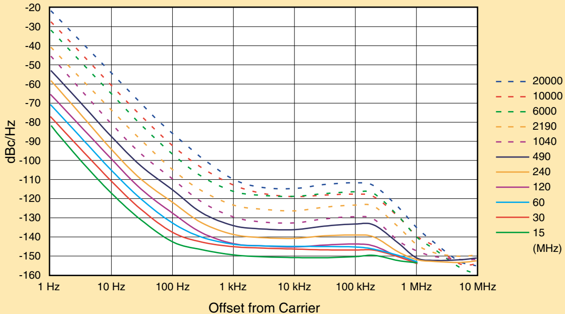
Typical SSB Phase Noise 69B with Option 21 DDC
